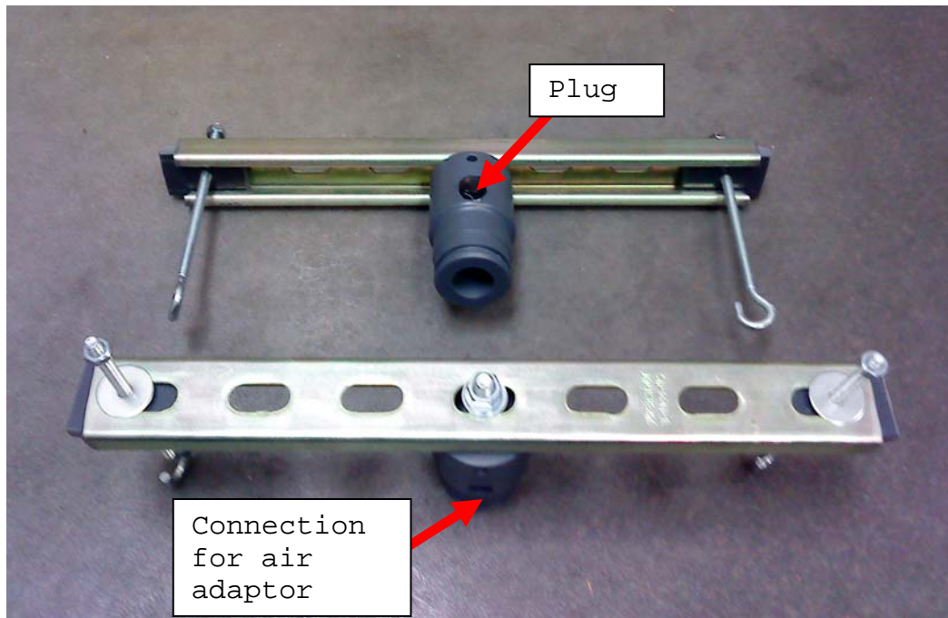
Figure 1: Assembly Kit of Hydraulics Bubble Test Apparatus
