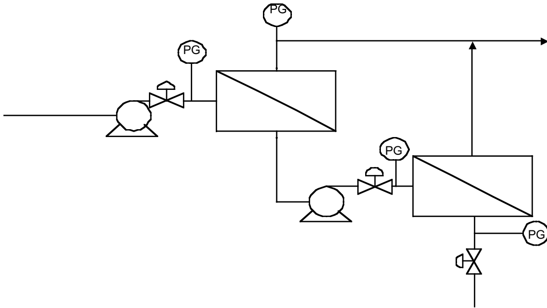
Fig 6. Flow diagram of an RO system with interstage booster pump
