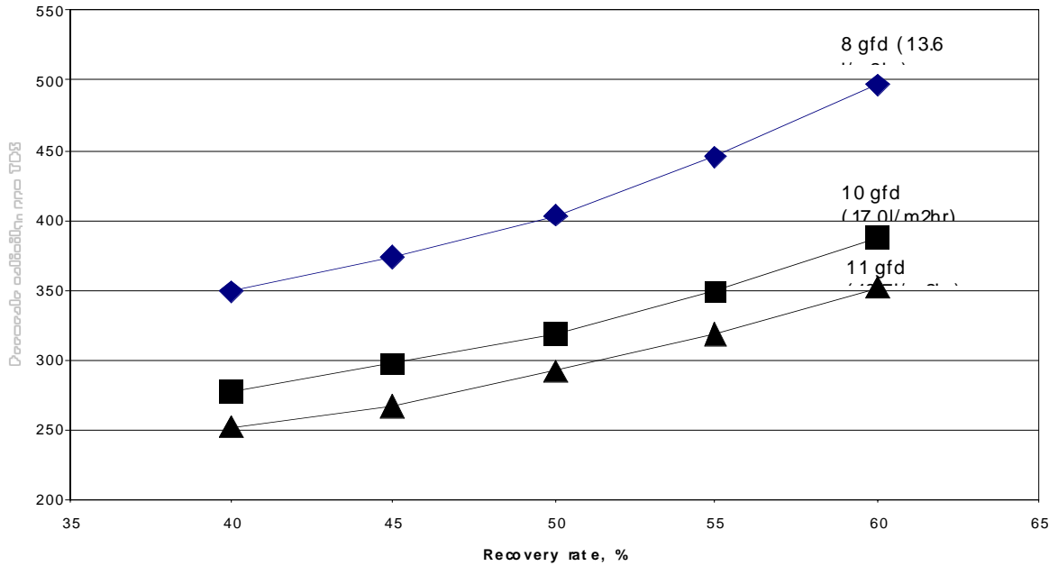
Fig 1. Projected permeate salinity for Mediterranean feed, ; at permeate flux rate range: 8 - 11 gfd
