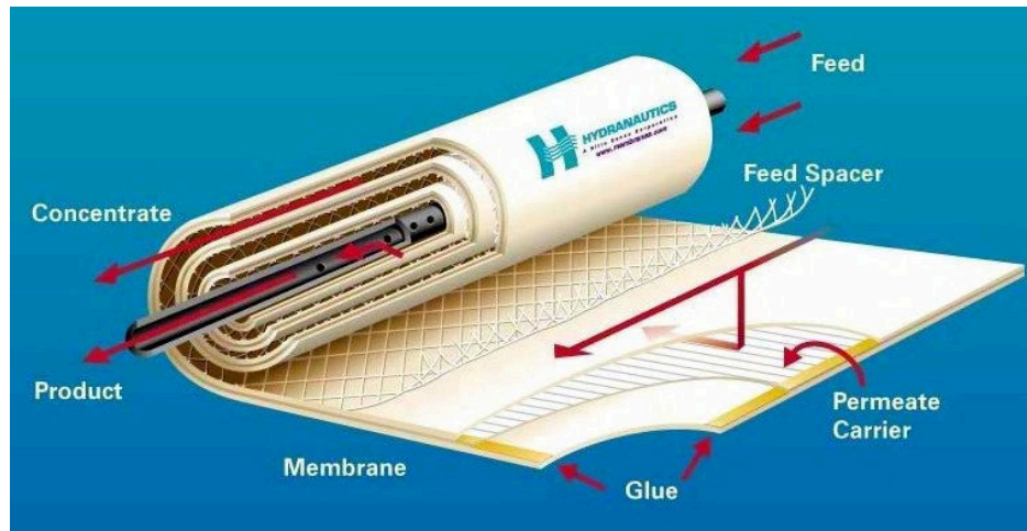
Figure 1: Typical Spiral Wound RO Element Components
