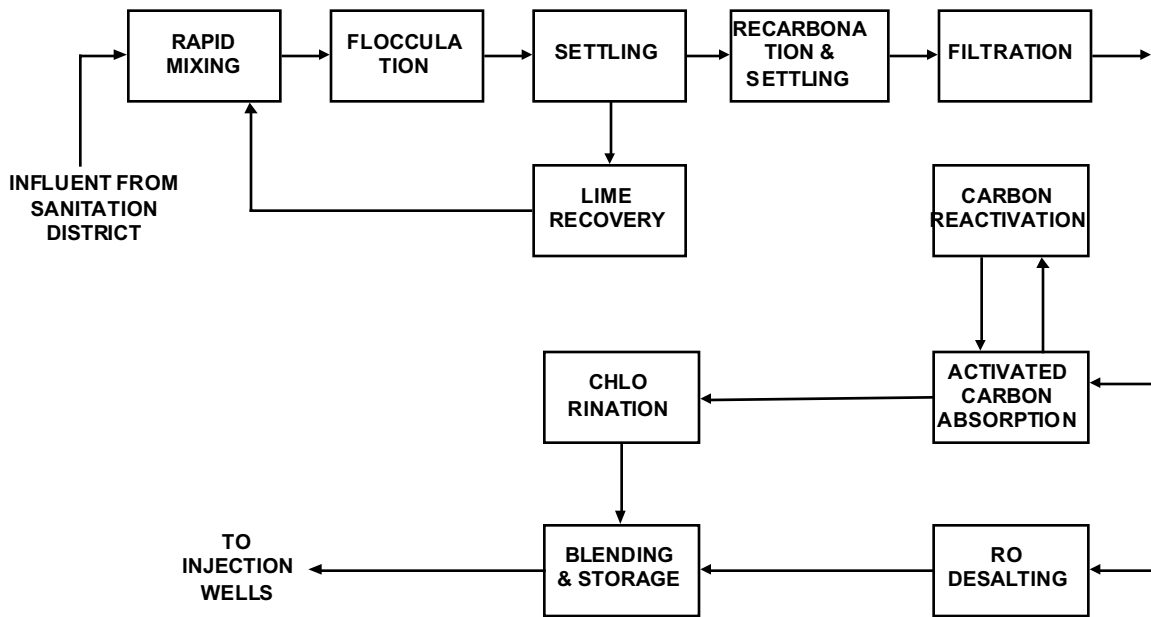
WATER FACTORY 21 WASTEWATER RECLAMATION SYSTEM FLOW DIAGRAM
