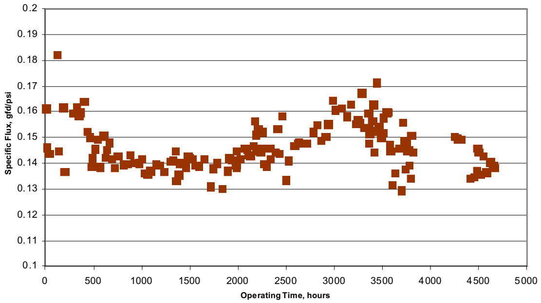
Figure 17-SAN PASQUAL SITE Wastewater Effluent, Capillary UF Pretreatment LFC1 Membrane Elements, Apr98 to Nov98
