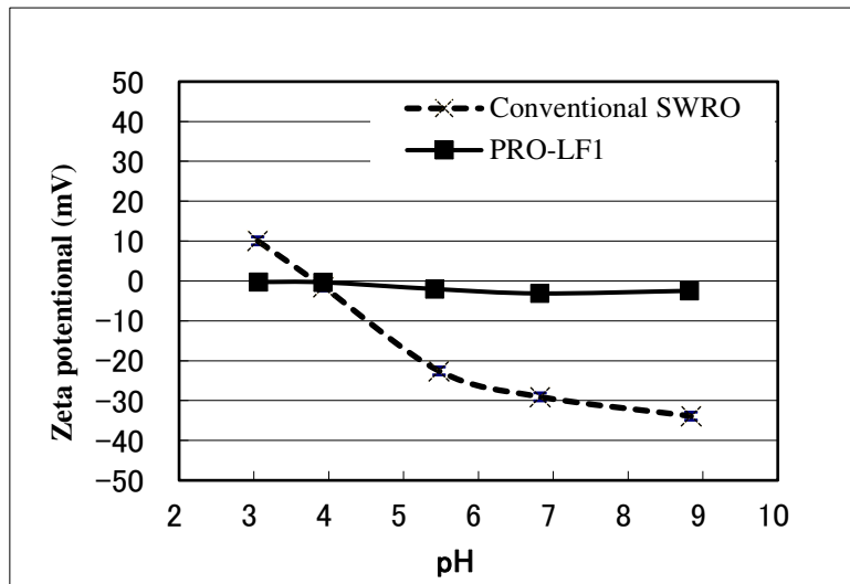
Figure 2 Effect of pH on the zeta potential of the membrane surface
