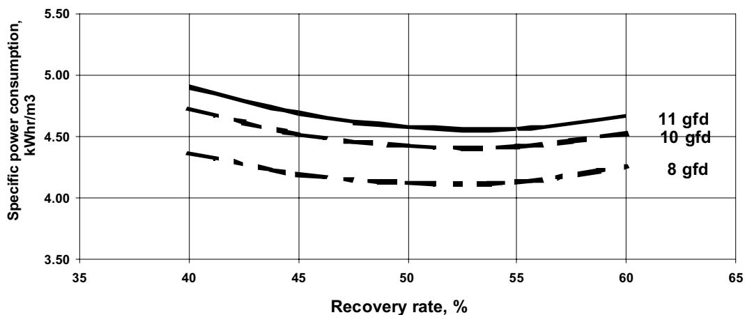
Fig 2. Projected power consumption for Mediterranean feed, 18 C
