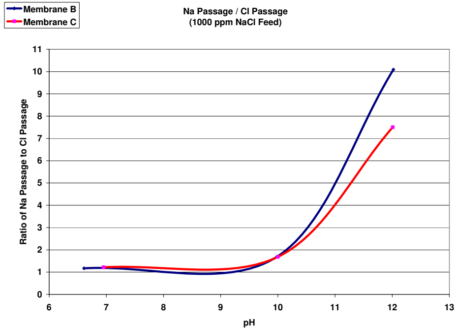
Figure 6. Ratio of sodium passage to chloride passage as a function of pH in two different membrane types. Test was done on single element at a flux of 15 gfd and at T = 25\text{ C} and a solution of 1000 ppm NaCl. Caustic soda was dosed to increase pH.
