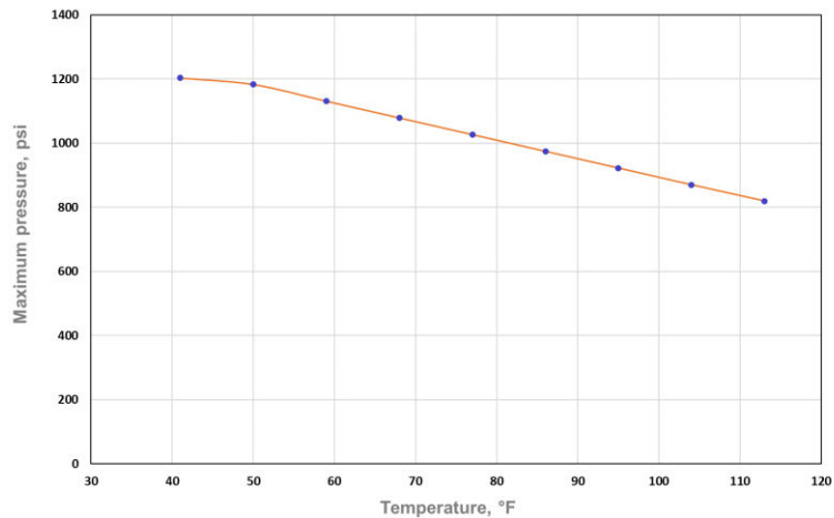
Maximum Membrane Feed Pressure vs Temperature Operational Curve
