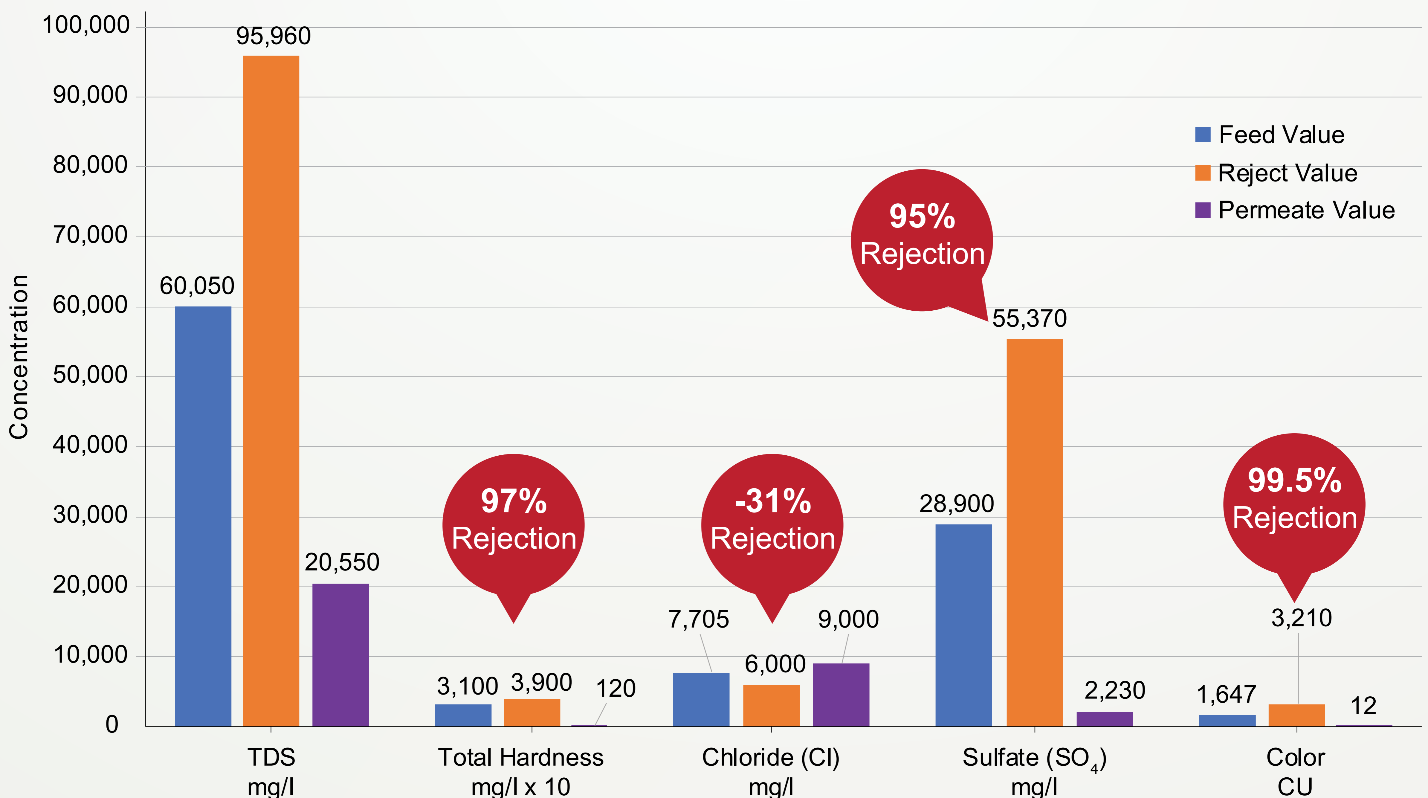
Field Testing Results for PRO-XS1 on Textile Wastewater Concentration of various components in Reject and Permeate Streams
