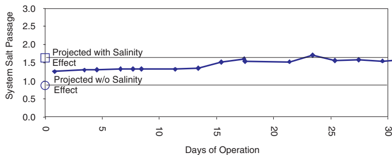
Fig. 9. Thirty days of normalized salt passage for a full scale RO system compared to projected salt passage with and without the 1.75 salinity factor.
