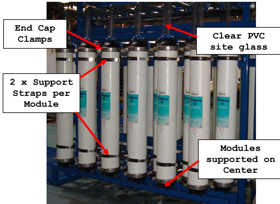
Figure 3: System design example with straps, site glass and well supported.
