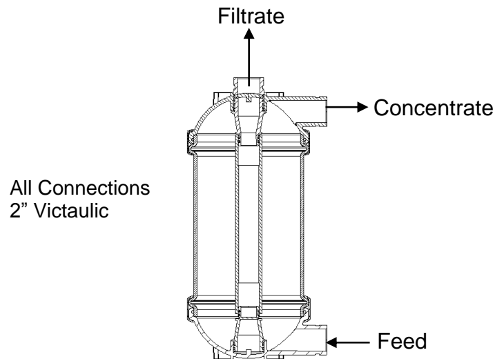
Figure 1: Flow Orientation
